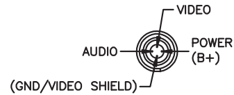
VIEW E-E SHOWN FROM PIN VIEW
